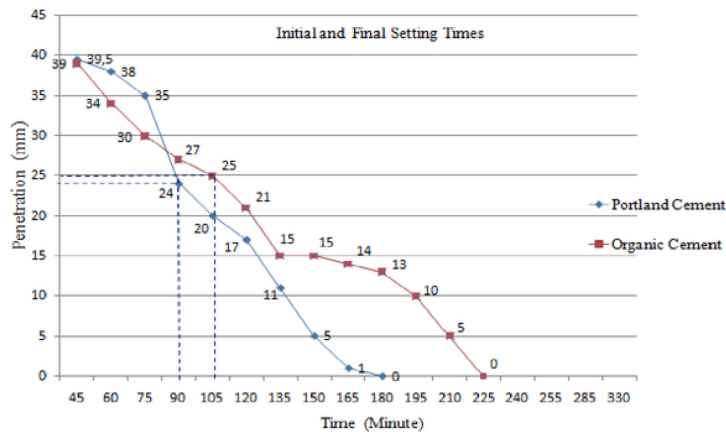
Figure 2 Initial and final setting time Graph
